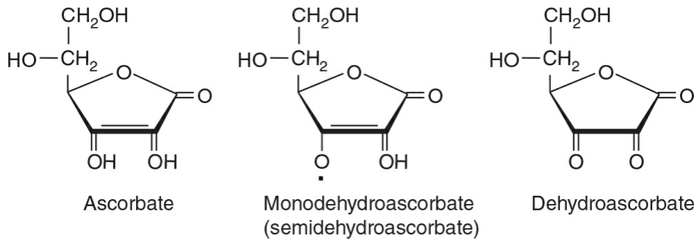
FIGURE 44–16 Vitamin C.
