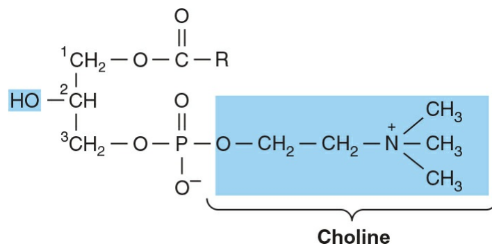
FIGURE 21–12 Lysophosphatidylcholine (lysolecithin).
