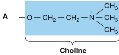
Phosphatidic acid
