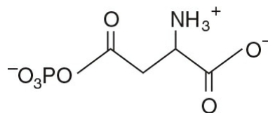
FIGURE 27-6 Aspartyl phosphate.
