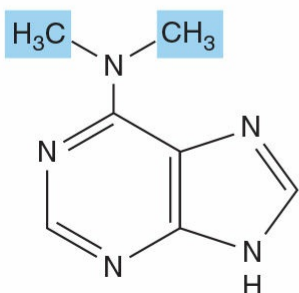
Dimethylaminoadenine
