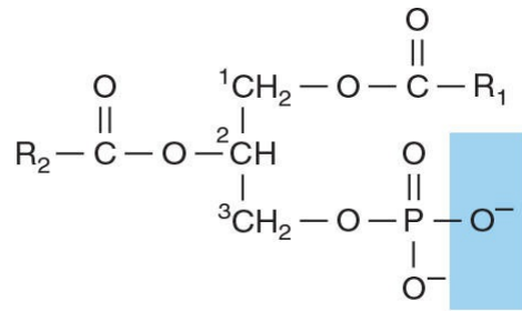
Phosphatidic acid
