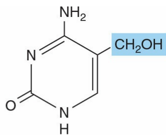
5-Hydroxymethylcytosine
