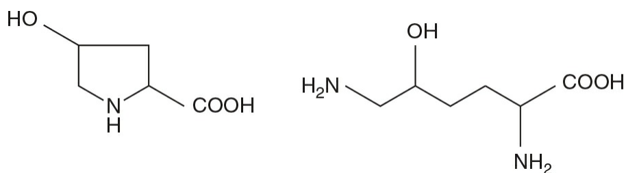
FIGURE 3–2 4-Hydroxyproline & 5-hydroxylysine.
