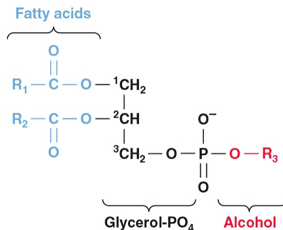
FIGURE 40–2 A phosphoglyceride showing the fatty acids ( \text{R}_1 and \text{R}_2 ), glycerol, and a phosphorylated alcohol component. Saturated fatty acids are usually attached to carbon 1 of glycerol, and unsaturated fatty acids to carbon 2. In phosphatidic acid, \text{R}_3 is hydrogen.
