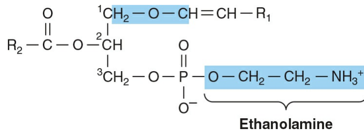
FIGURE 21–13 Plasmalogen.
