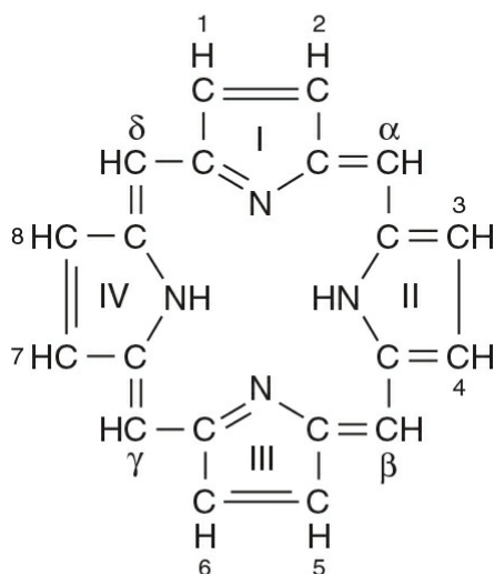
Porphyrin ( C_{20}H_{14}N_4 )
