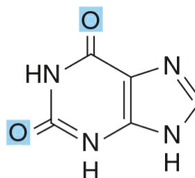
Xanthine (2,6-dioxypurine)
