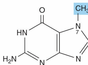
7-Methylguanine
