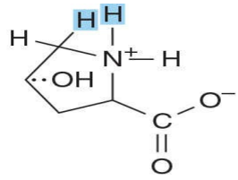
4-Hydroxy-L-proline
