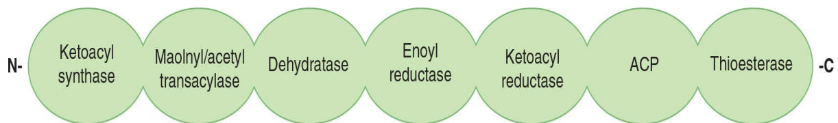
Sequence of enzyme domains in primary structure of fatty acid synthase monomer
