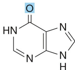
Hypoxanthine (6-oxopurine)
